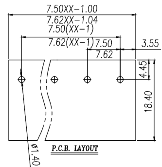
PCB开孔图 PCB Opening diagram
