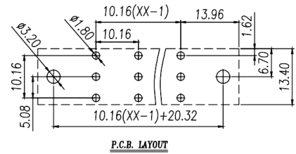
PCB开孔图 PCB Opening diagram
