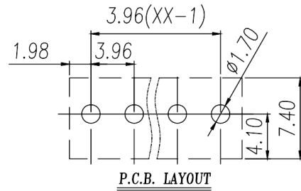
PCB开孔图 PCB Opening diagram
