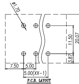
PCB开孔图 PCB Opening diagram
