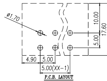
PCB开孔图 PCB Opening diagram
