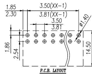
PCB开孔图 PCB Opening diagram
