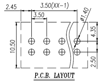
PCB开孔图 PCB Opening diagram
