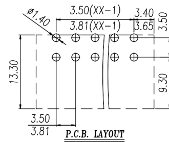
PCB开孔图 PCB Opening diagram
