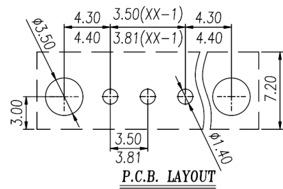
PCB开孔图 PCB Opening diagram
